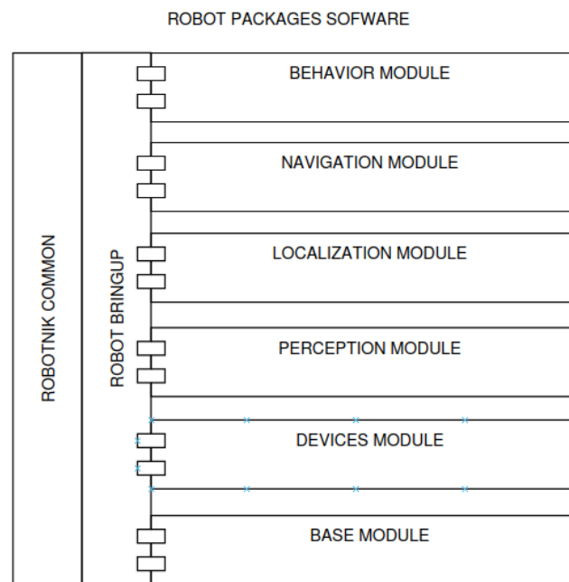
Figure - Robot Software Architecture
